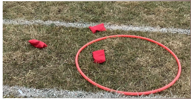
Accuracy
